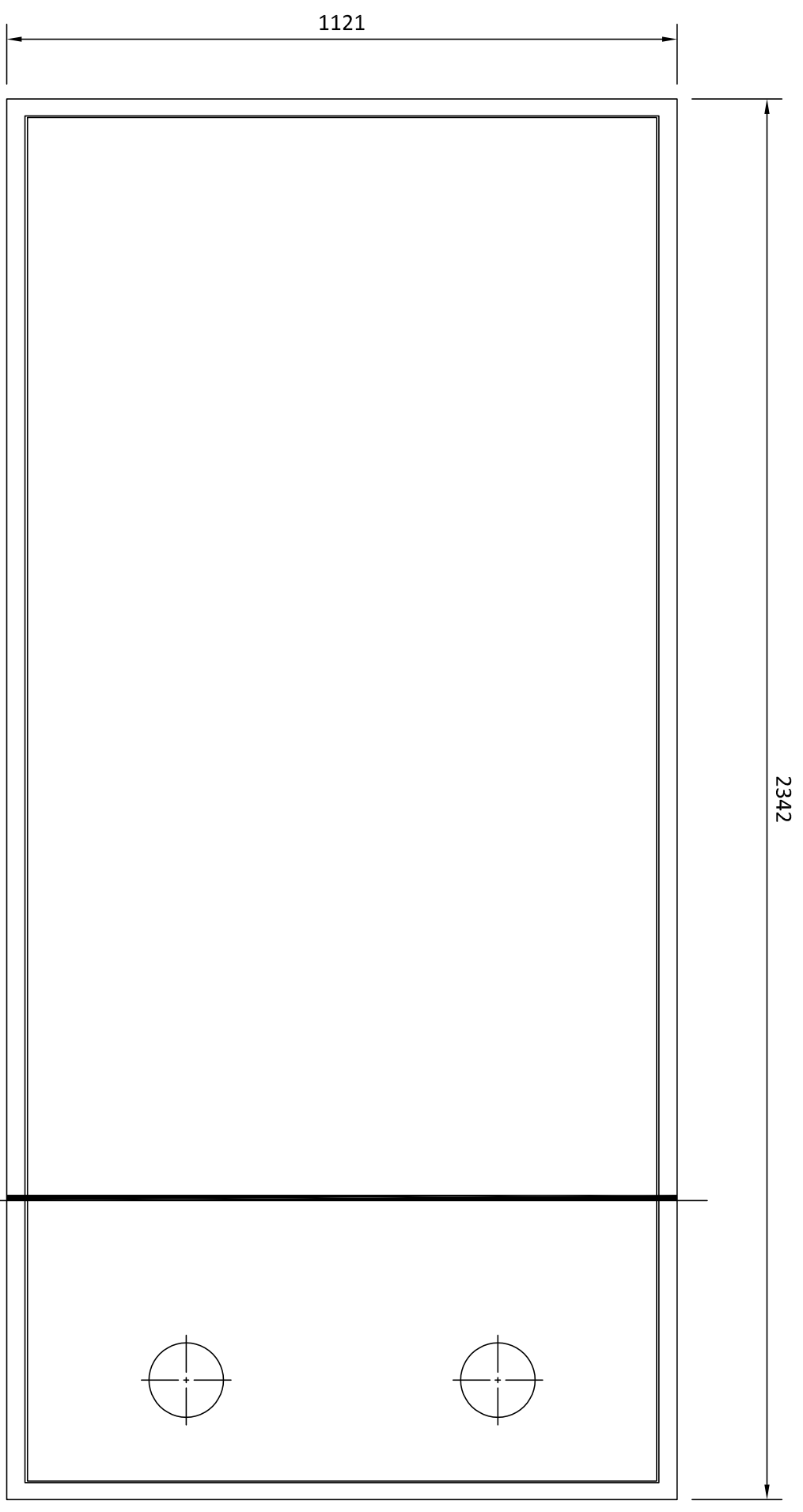
BASIC COLLECTOR FRAME ELEVATION
