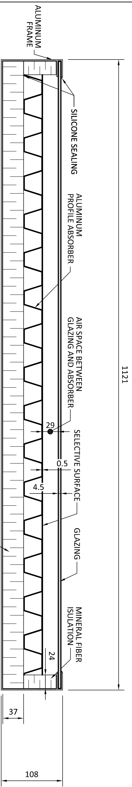
A FRESCO COLLECTOR DETAIL SCALE : 1:4
