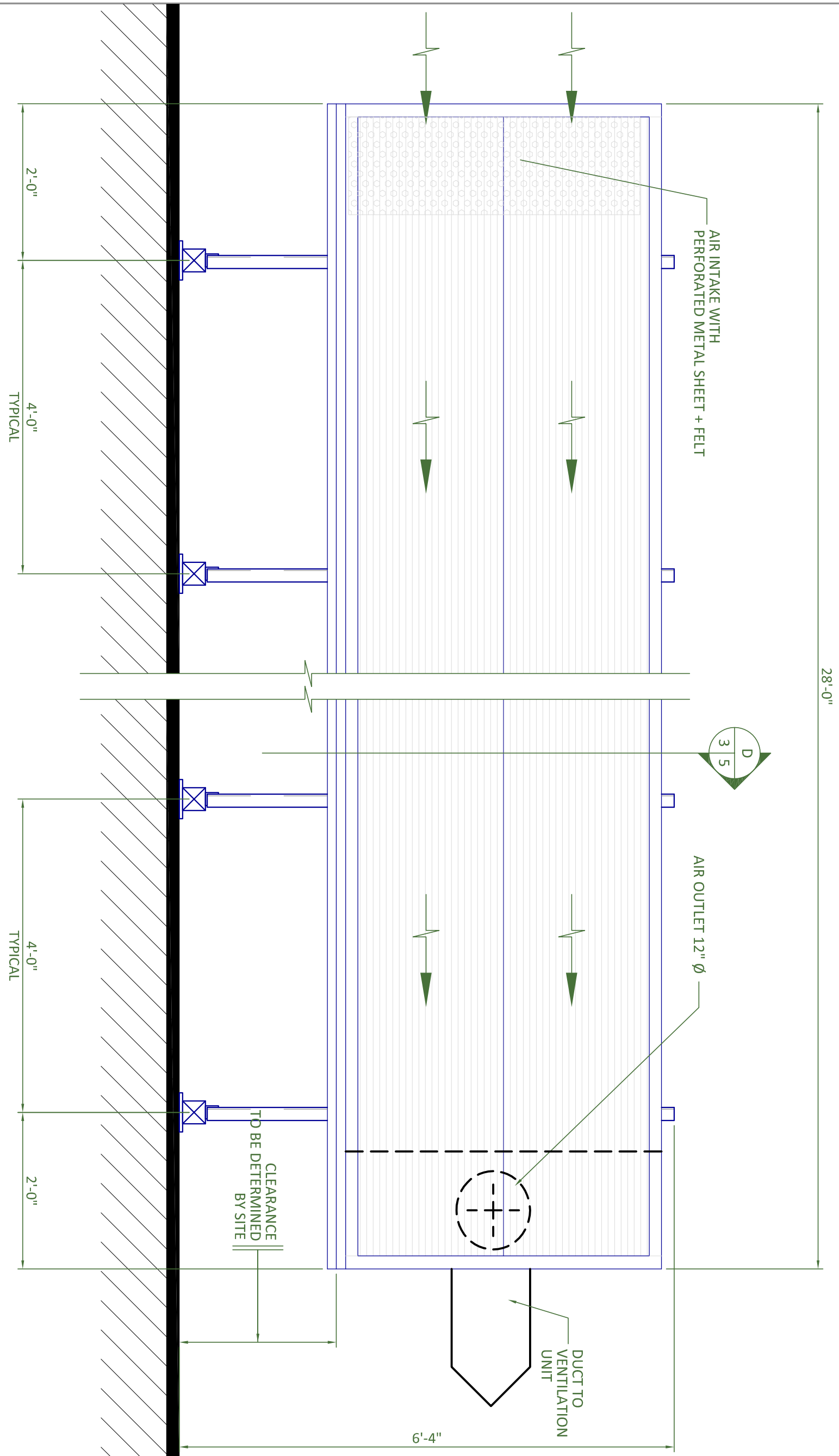
A ELEVATION VIEW OF DOUBLE FRESCO SYSTEM 2 | 3 SCALE : 3/4" = 1'-0"
